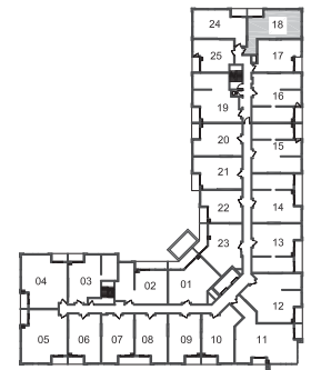
LEVEL 3-4
