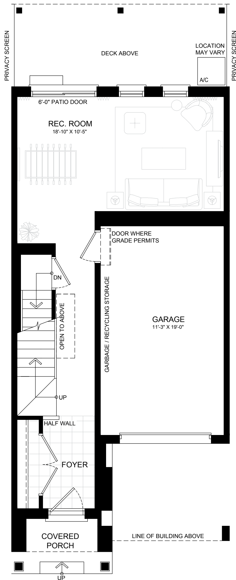
GROUND FLOOR
