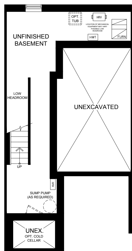
BASEMENT
