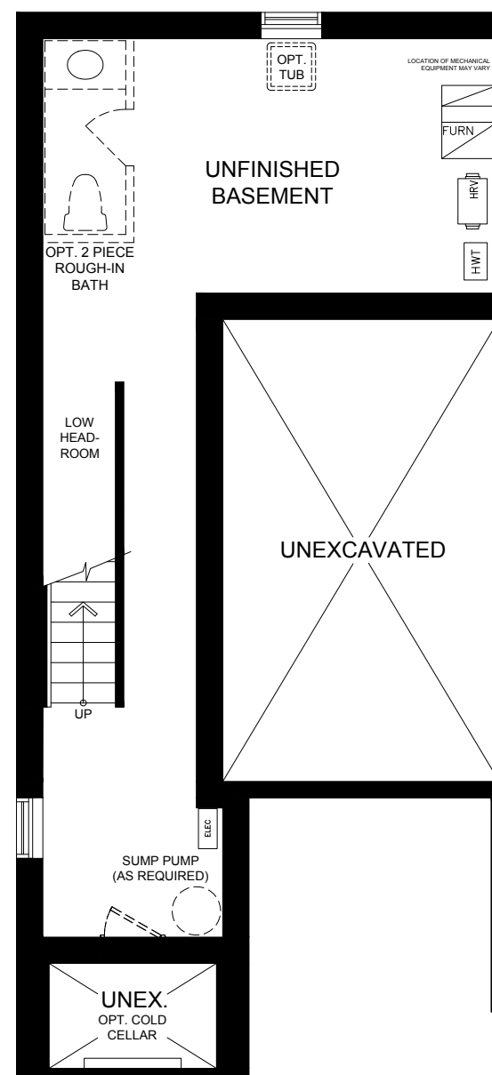
BASEMENT
