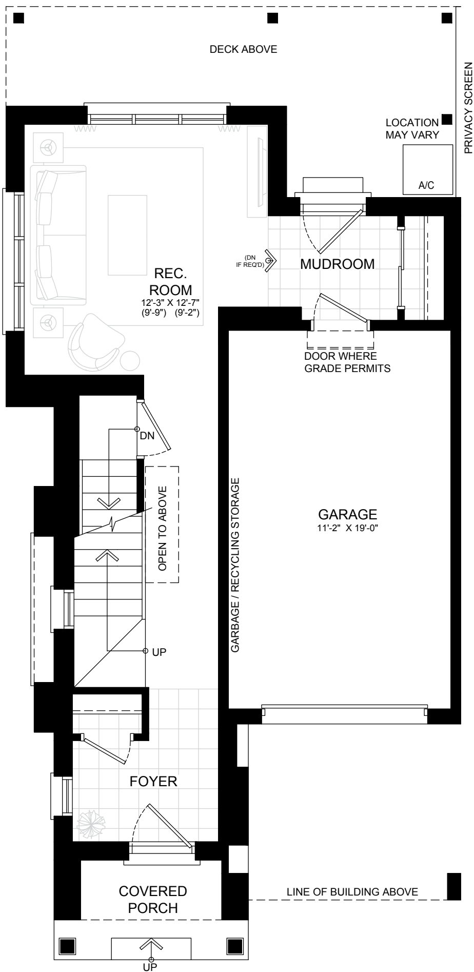
GROUND FLOOR
