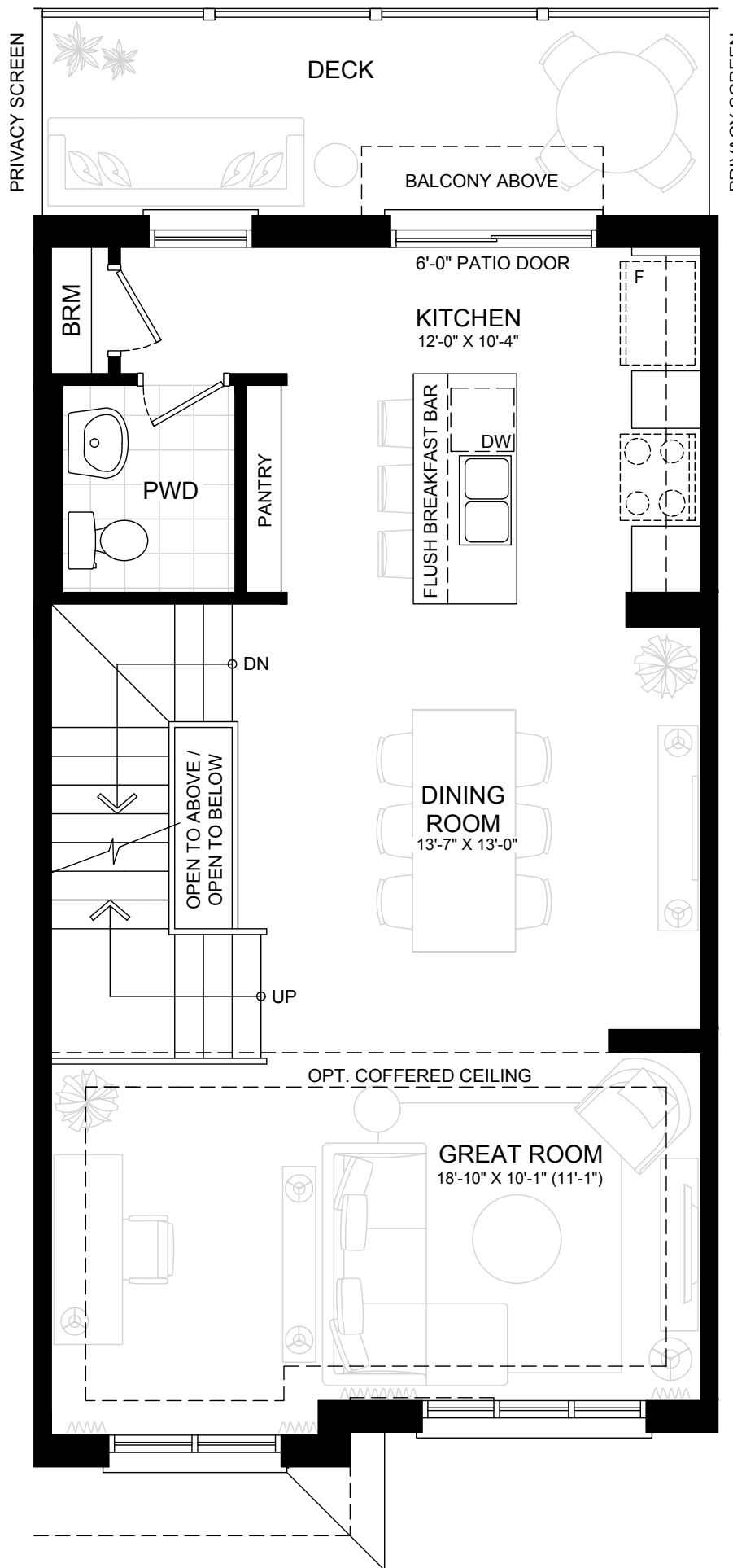
MAIN FLOOR
