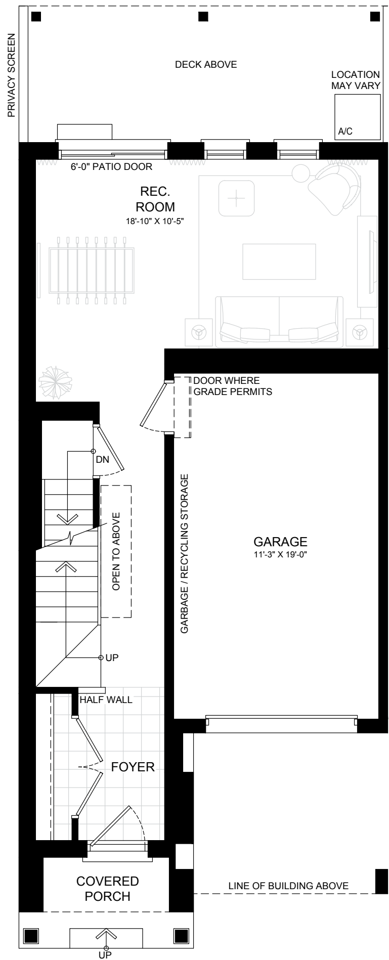
GROUND FLOOR
