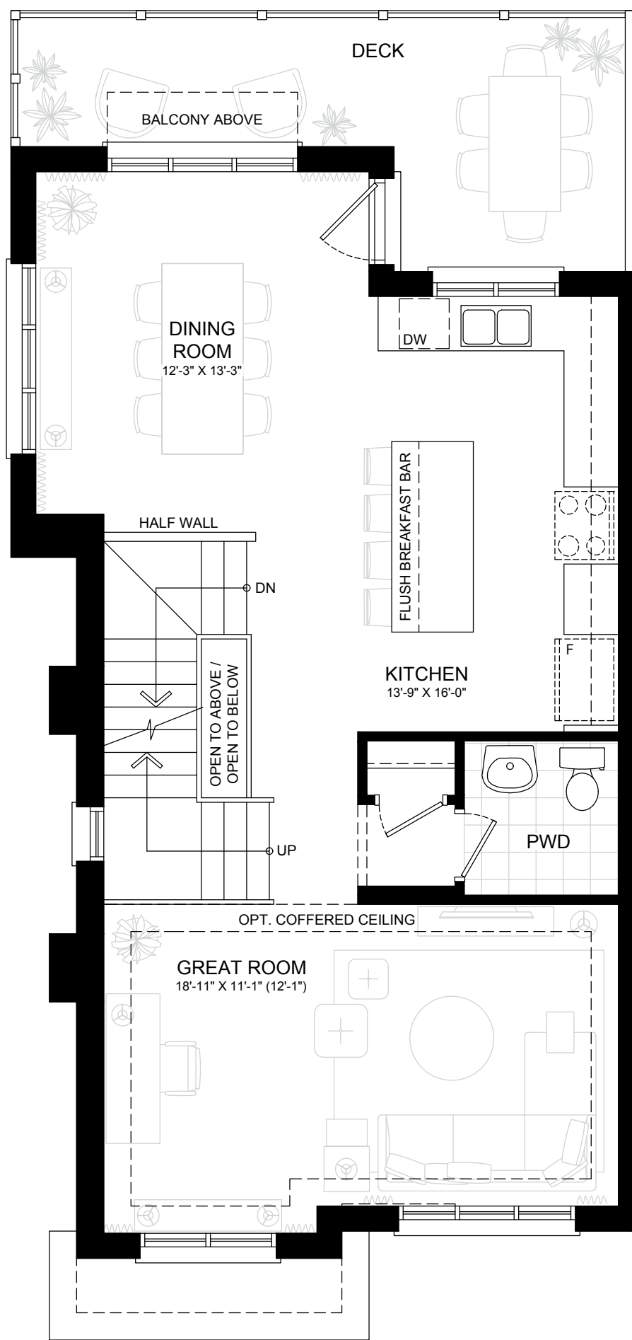
MAIN FLOOR
