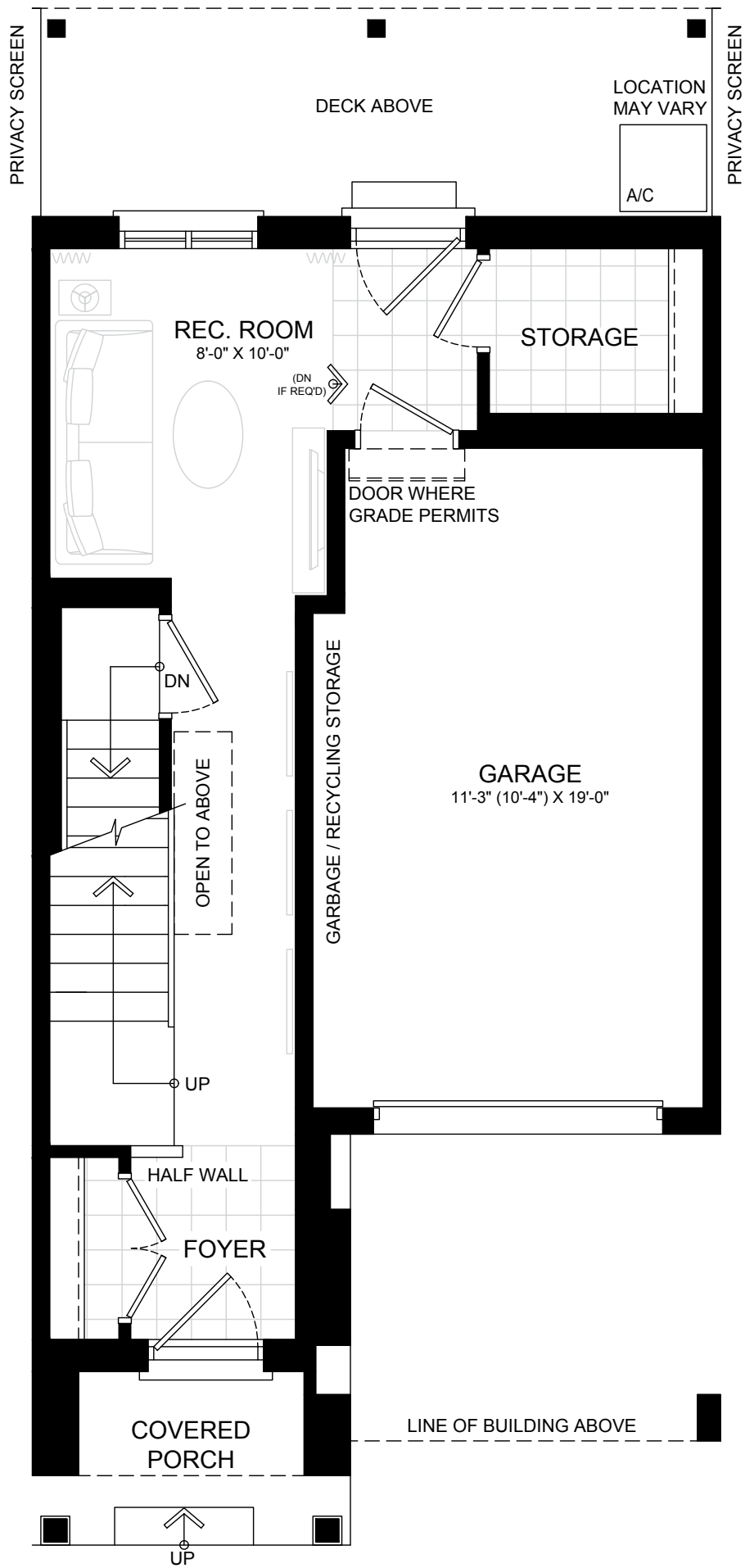
GROUND FLOOR
