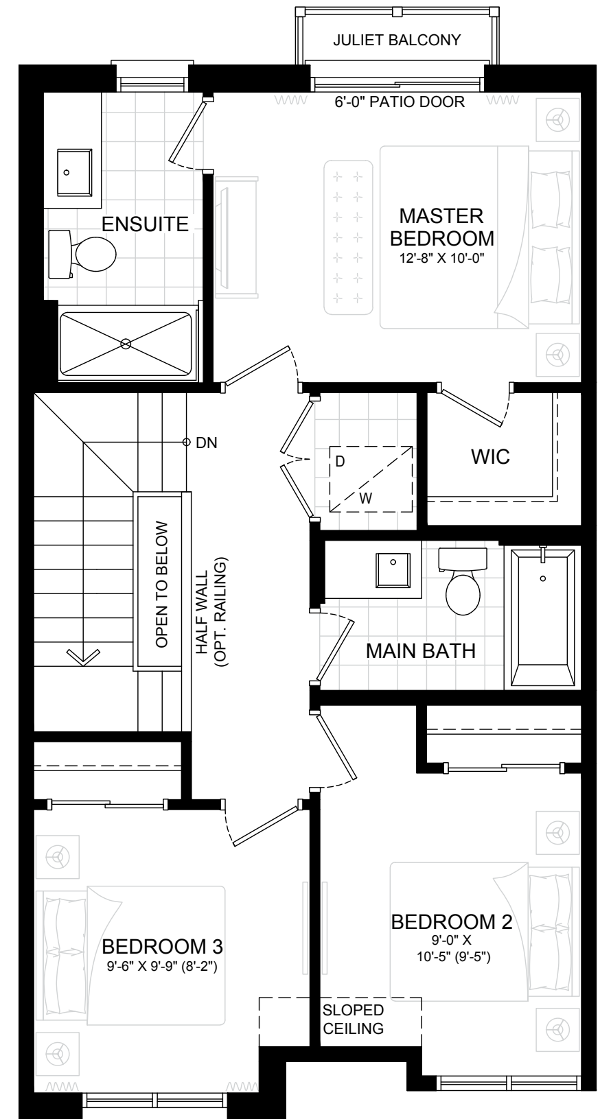
SECOND FLOOR
