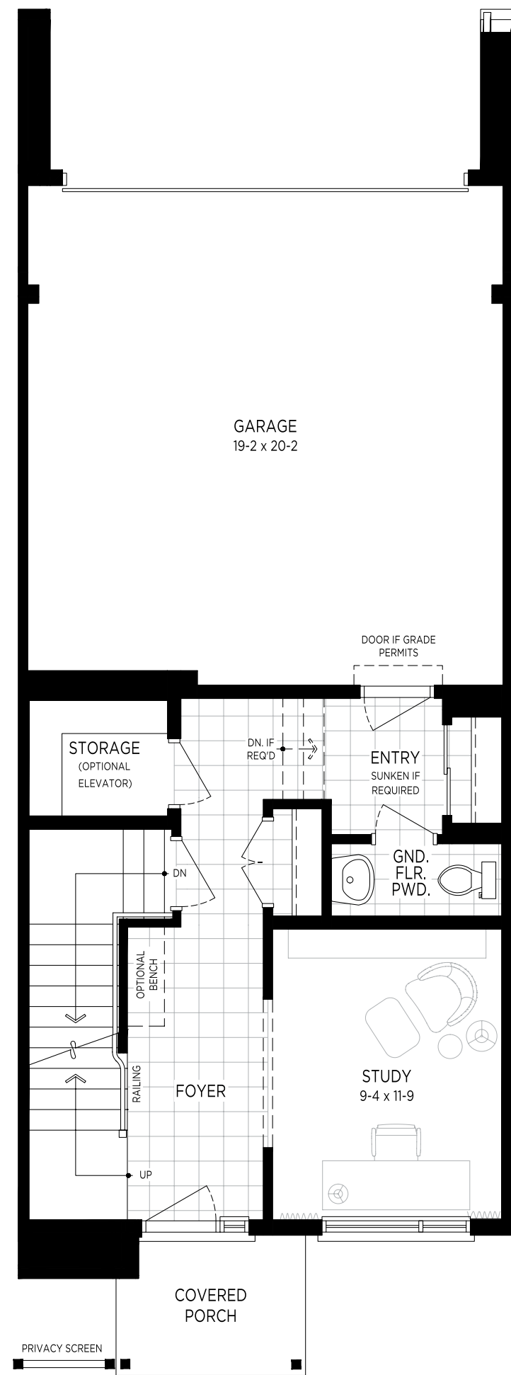
GROUND FLOOR
