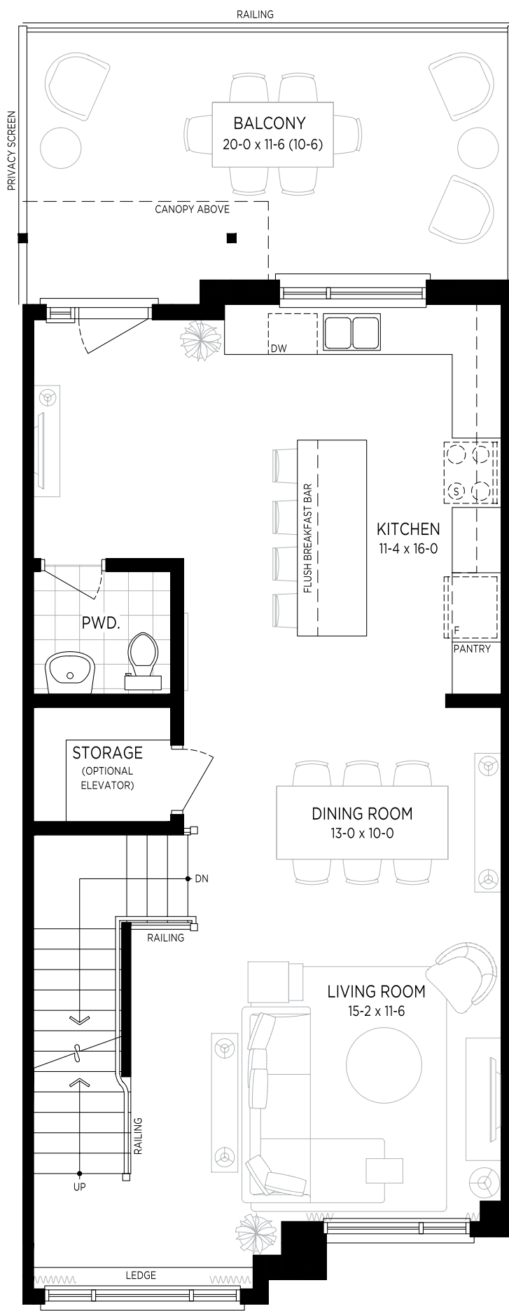
MAIN FLOOR
