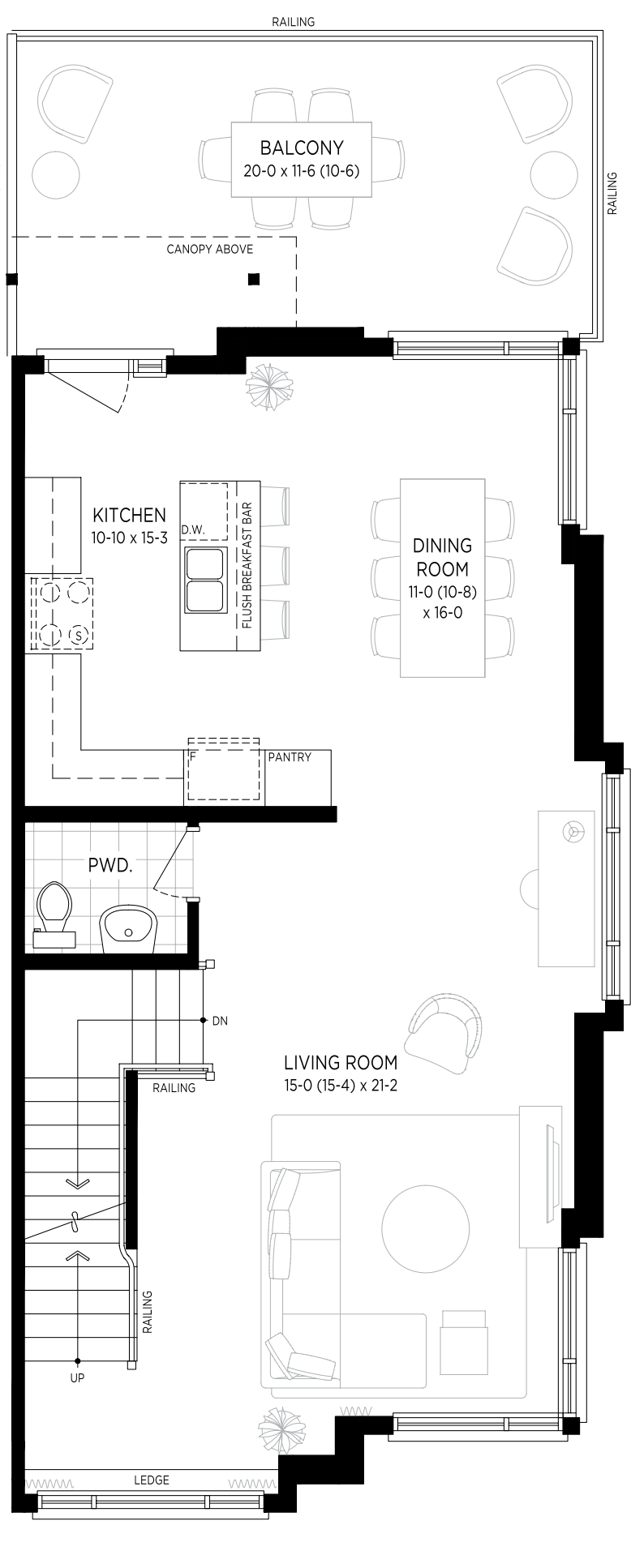
MAIN FLOOR
