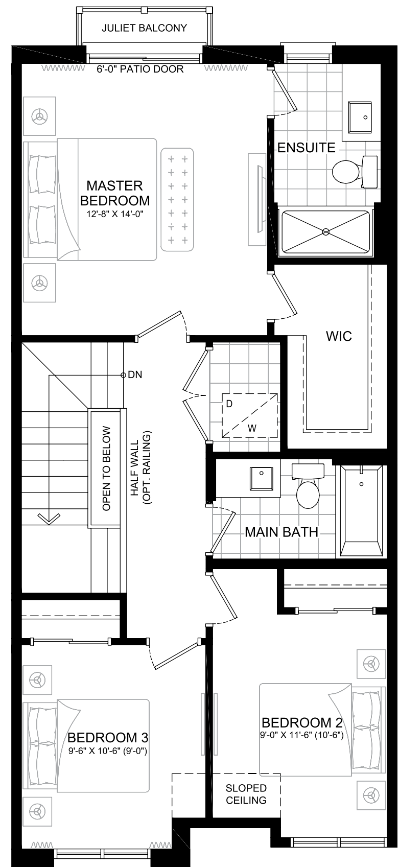
SECOND FLOOR
