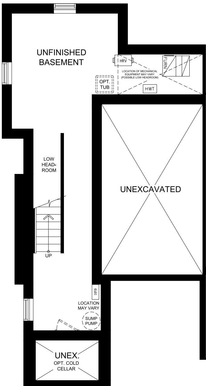
BASEMENT
