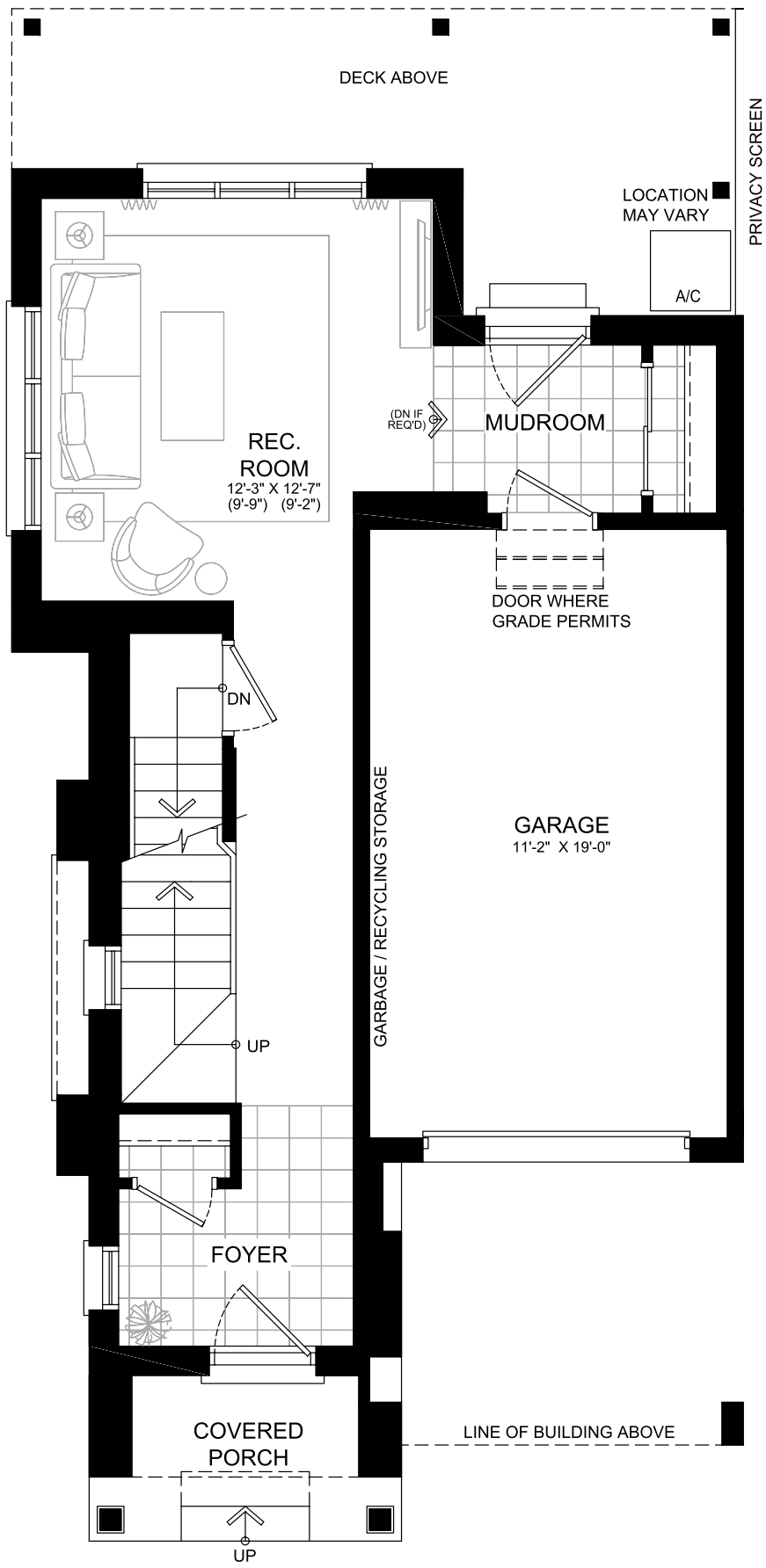
GROUND FLOOR
