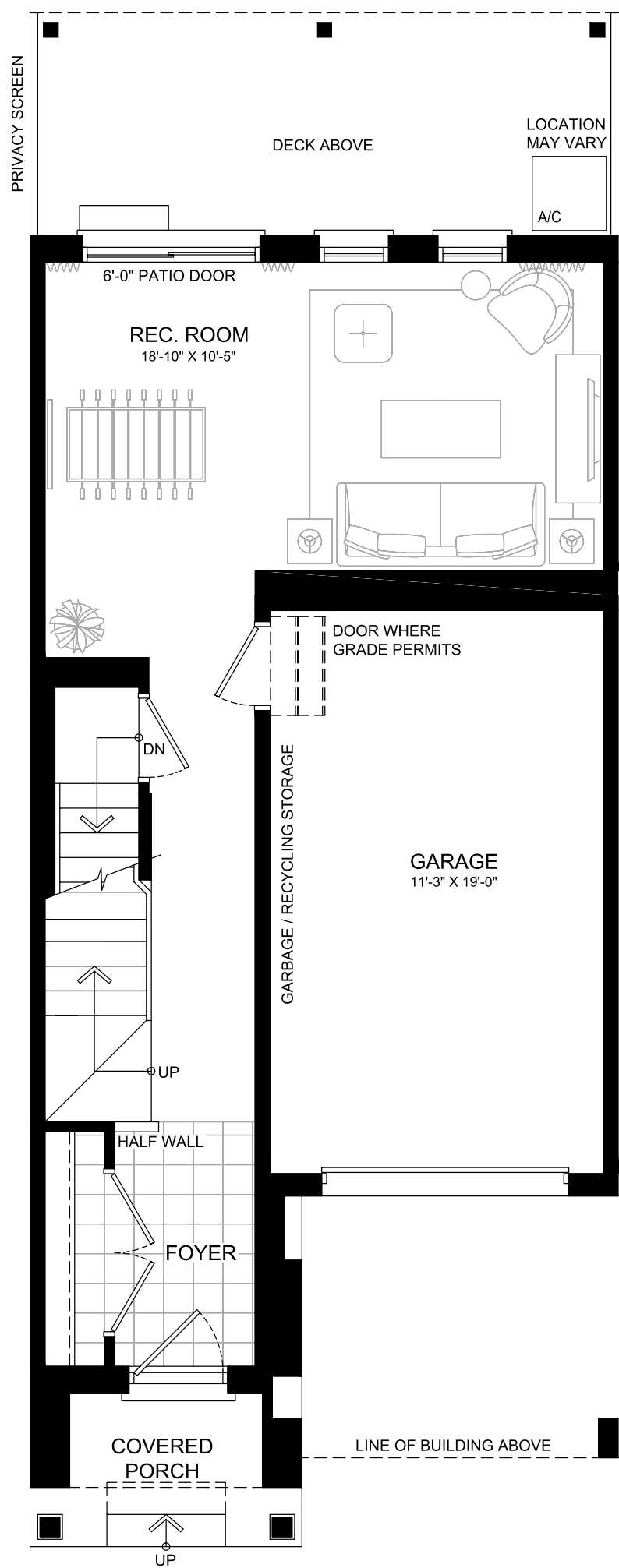
GROUND FLOOR
