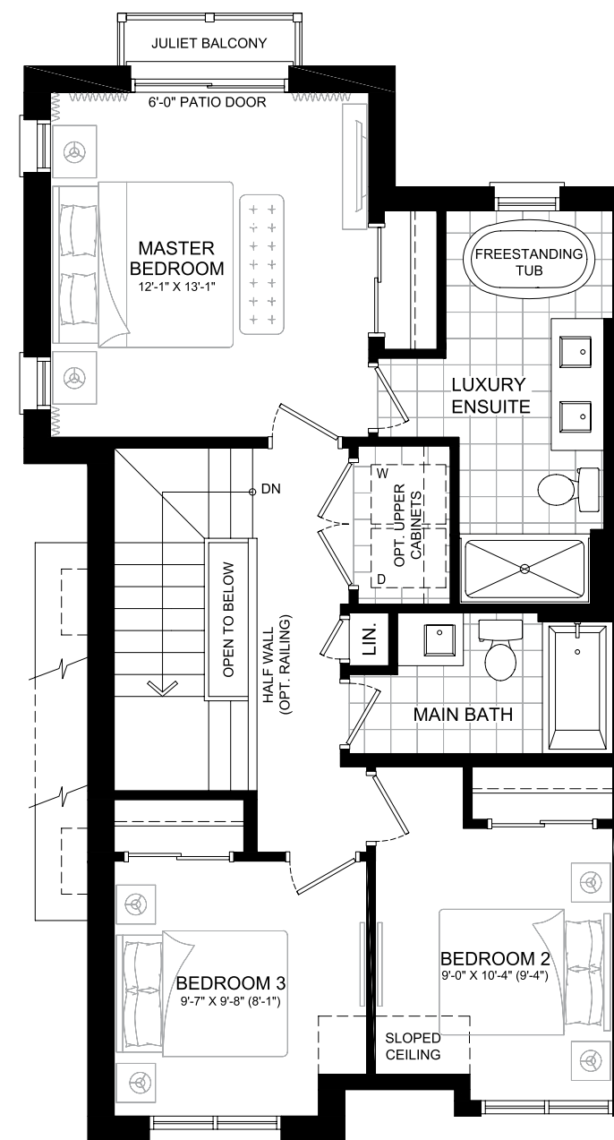
OPT. SECOND FLOOR
